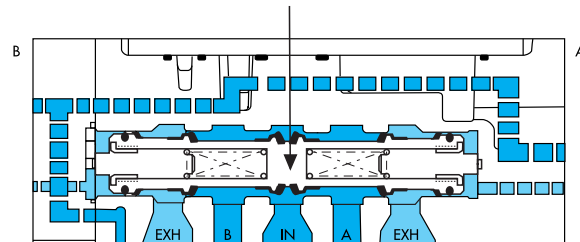
3 POSITION SINGLE PRESSURE, PRESSURE CENTER
