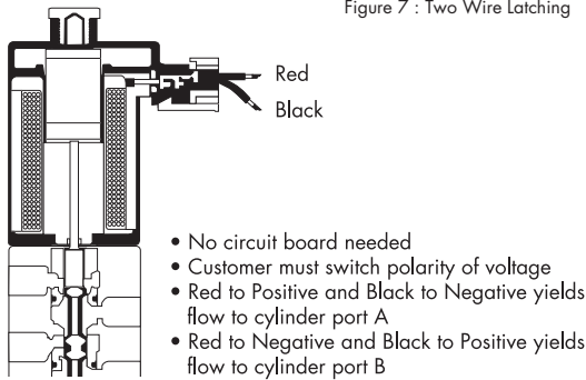
Figure 7 : Two Wire Latching
