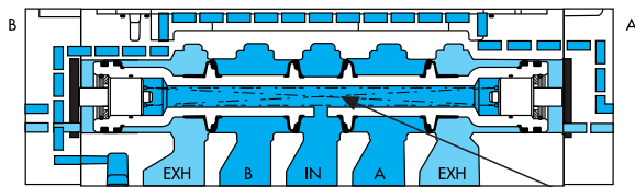
3 POSITION CLOSED CENTER
